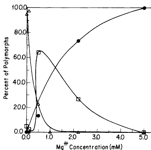
Figure 10. Effects of \text{Mg}^{2+} concentration on the yield of \text{CaCO}_3 polymorphs.
