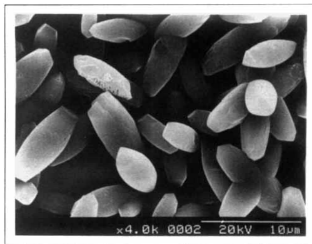
Figure 13. Football-shape calcite.
