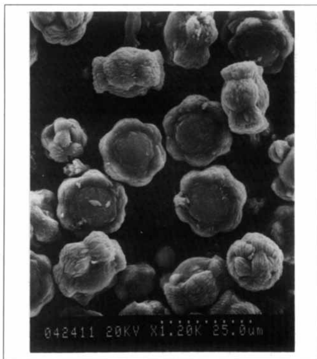
Figure 17. Hexagonal-plate vaterite.
